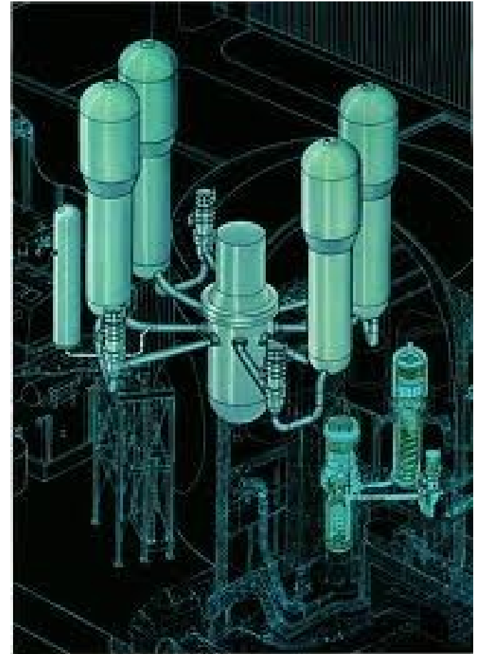
Westinghouse BWR666 STEAM SUPPLY SYSTEM
